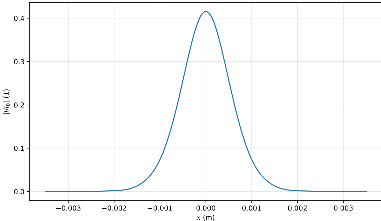
Intensity profile I(x, y = 0, z = 3.821m)/I_0 , P_{in}=0.5P_{cr} , artificial time
